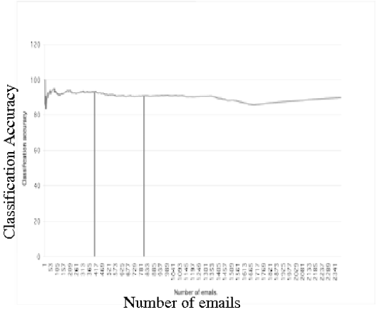
Fig. 6. The modified system is capable of maintaining classification accuracy as the user preferences for a particular set of emails change from interesting to uninteresting (first vertical line) and then back to interesting again some time later (2nd vertical line)
