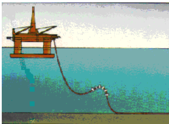
Fig. 1. Lazy-wave Configuration
