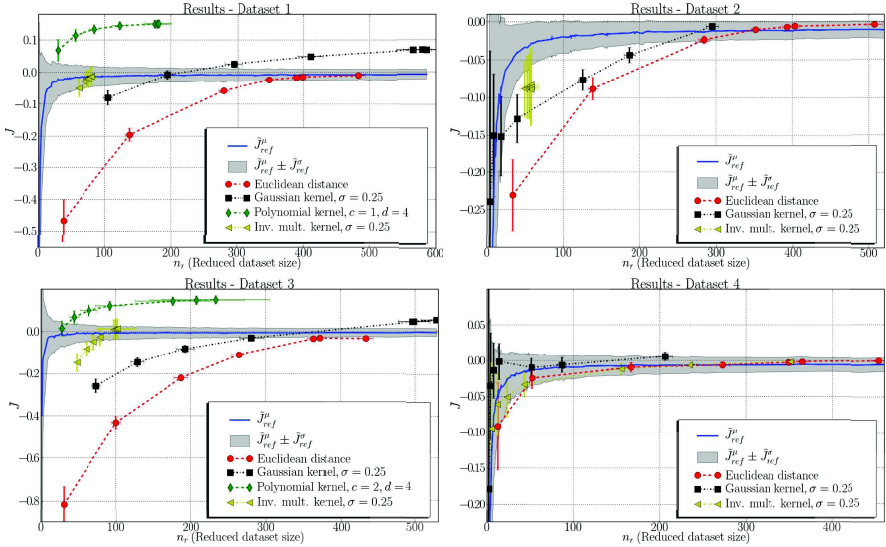
Fig. 1. Obtained results for different distance functions in the four synthetic datasets. \bar{J}_{ref}^\mu and \bar{J}_{ref}^\sigma denote the mean and standard deviation of the reference entropy values, respectively.
