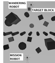
Fig. 2. Simulated World 2
