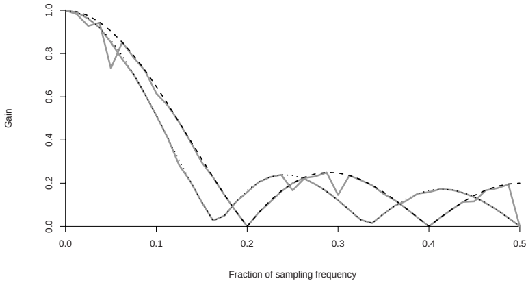
Fig. 5. The frequency responses of the single cell models for a migration threshold of 90 and 110. The dotted-line illustrates M_i = 90 and the dashed-line illustrates M_i = 110 . In both cases the corresponding solid, grey line is the actual response.
